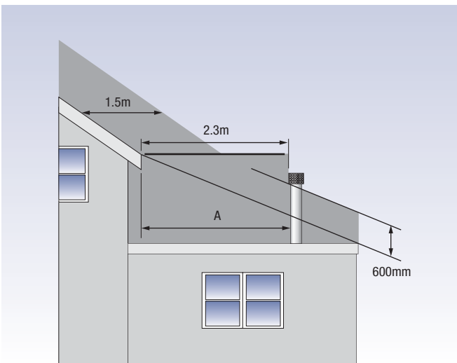
The flue shall terminate outside the dark shaded zone.
