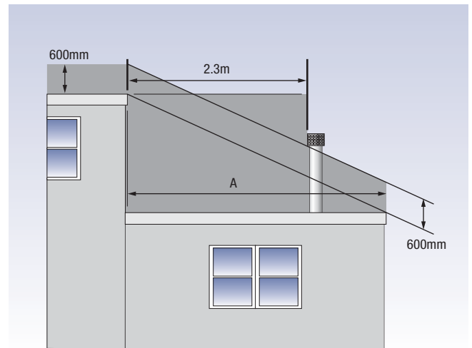
The flue shall terminate outside the dark shaded zone.
