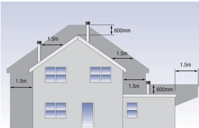
The flue shall terminate outside the dark shaded zone.
