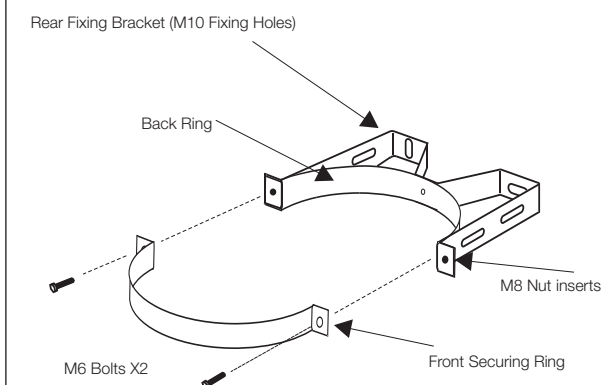
Fig. 3 Wall Band Assembly
