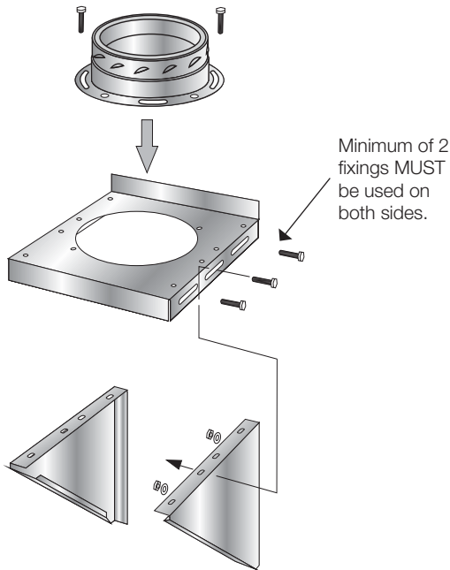
Fig. 4 Wall Support Assembly
