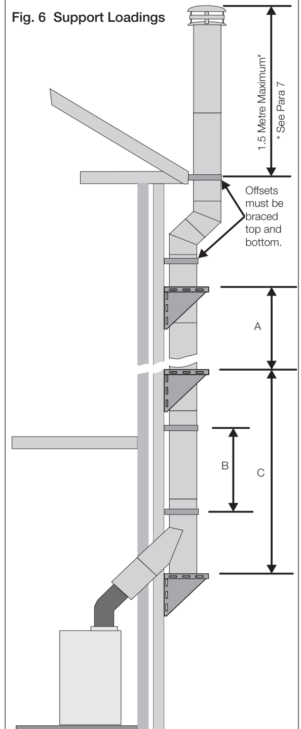
Maximum Wall Support Clearances for Fig. 5.
