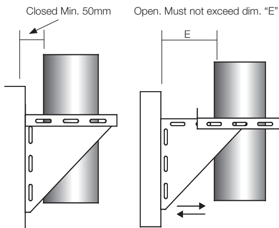
Fig. 5 Wall Support Assembly Clearance
