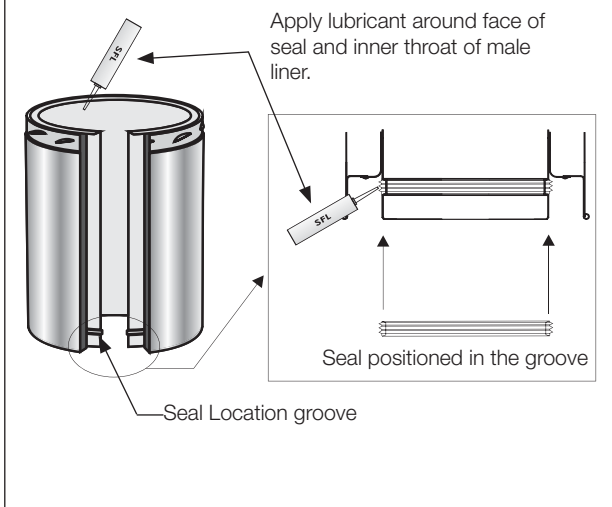
Fig. 8 Seal Installation
