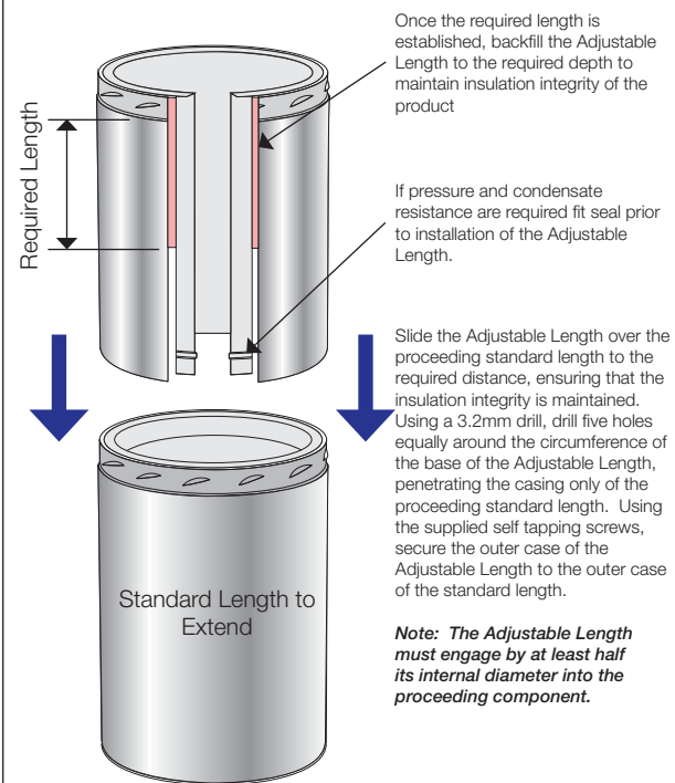
Fig. 2 Adjustable Length Assembly
